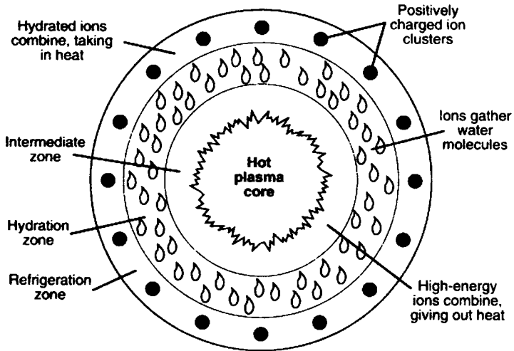
Fig. 6 The structure of ball-lightning. (After David Turner, New Scientist , 20 March 1993)
