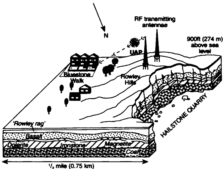
Fig. 16 Geophysical representation of the Hallstone Quarry area, Rowley Regis, showing the radio antennae and the trajectory of an earthlight UAP to Jean Hingley's house in Bluestone Walk.
